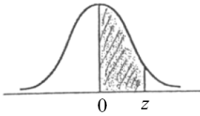
Normal Probabilities
